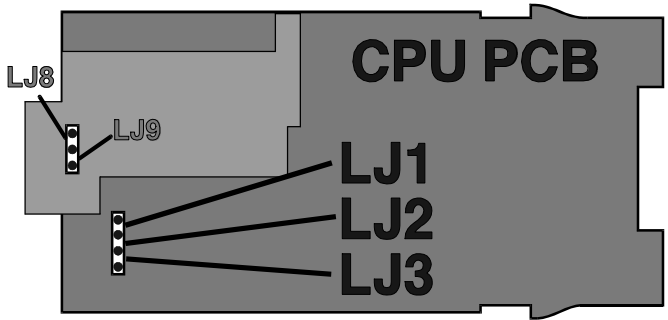
Figure 2 1/16-DIN Link Jumpers (DC Output 1)
