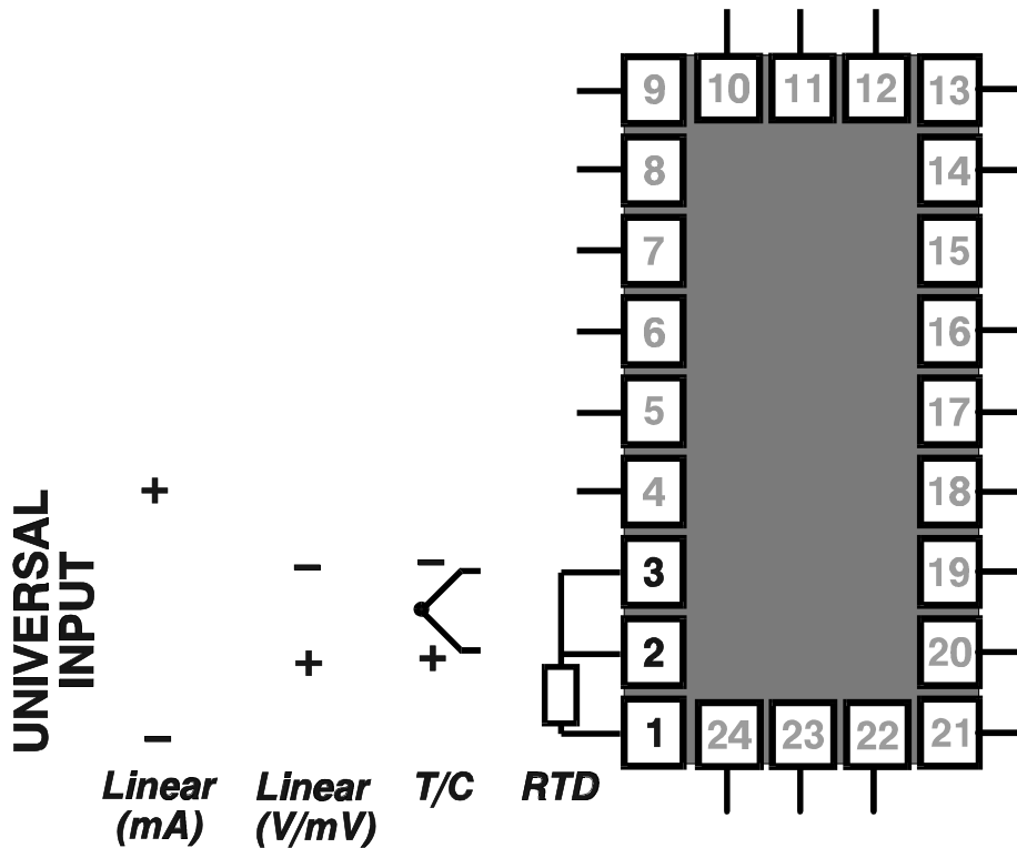
Figure 5 1/4-DIN/1/8-DIN Universal Input Connections
