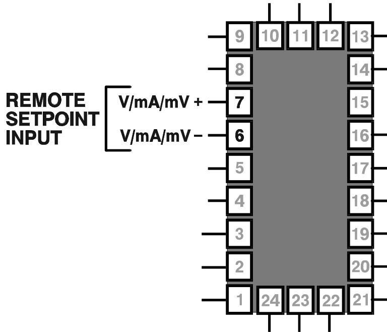
Figure 6 \frac{1}{4} -DIN/ \frac{1}{8} -DIN Controllers - Secondary Analogue Input
