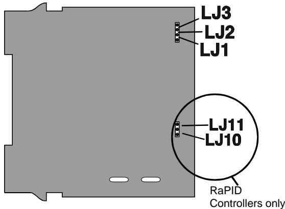
Figure 3 1/4-DIN/1/8-DIN Series Link Jumpers
