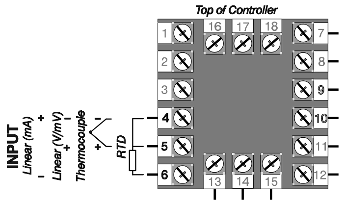
Figure 4 1/16-DIN Universal Input Connections
