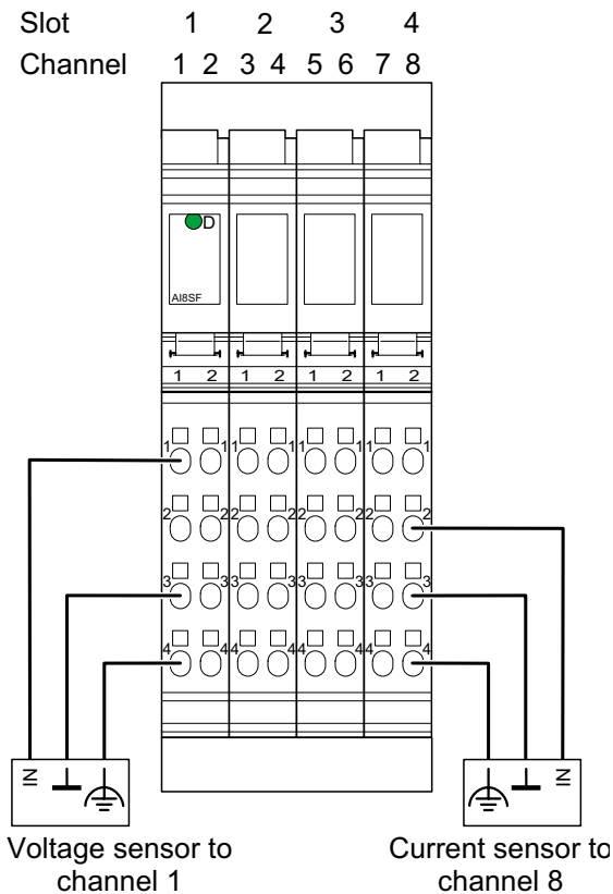
Figure 5 Connection of active sensors using 2-wire technology with shield connection
