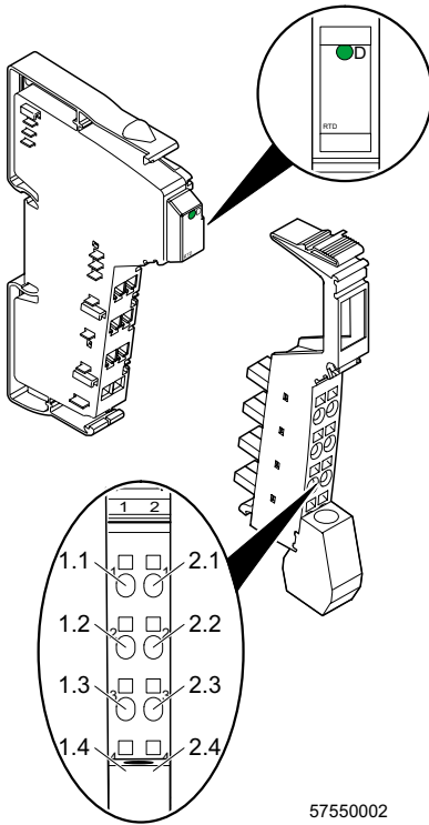
Figure 2 VARIO RTD 2 with the appropriate connector
