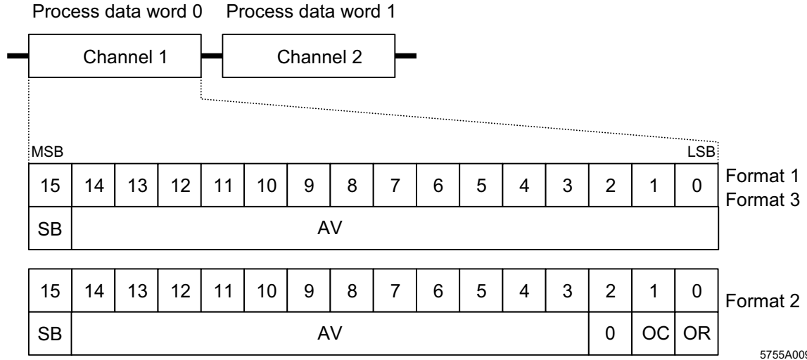
Bild 8 Sequence of the process data input words and representation of the bits of the first process data word in different formats
