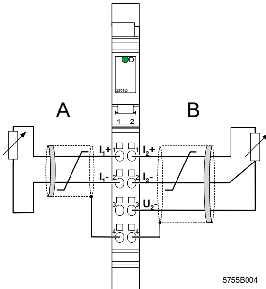
Figure 5 Sensor connections in 2- and 3-wire technology with shield connection
