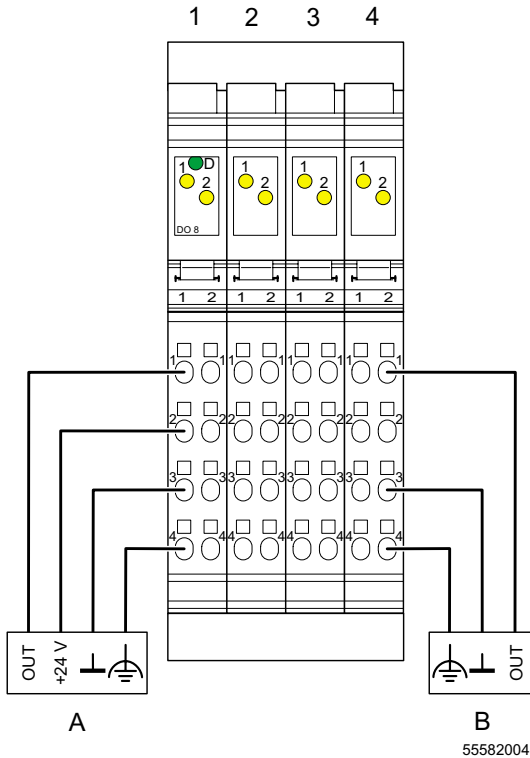
Figure 4 Typical actuator connections
