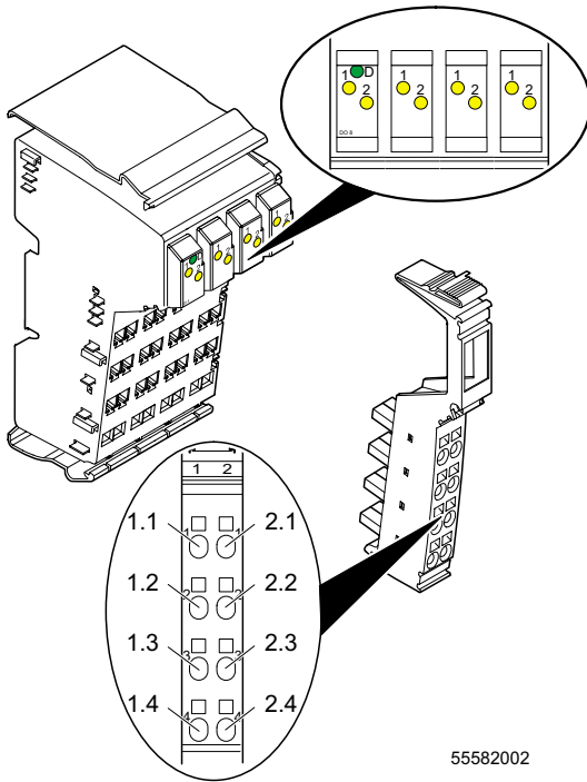
Figure 2 VARIO DO 8/24 with appropriate connectors
