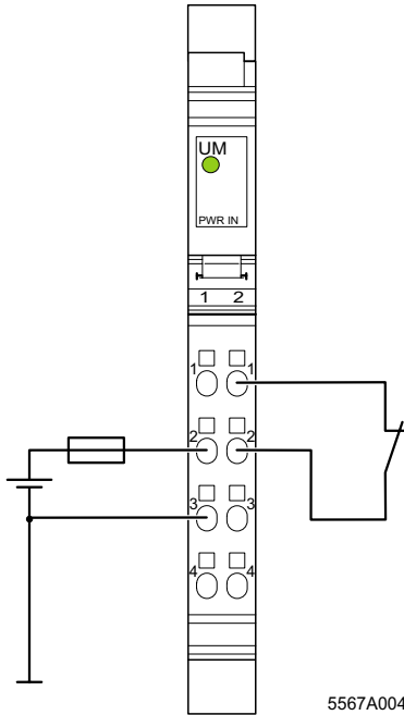
Figure 4 Typical connection of the supply voltage U_M and of an external switch to supply the segment voltage U_S
